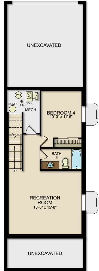
Opt. Lower Level Floor Plan 600 Sq.ft
