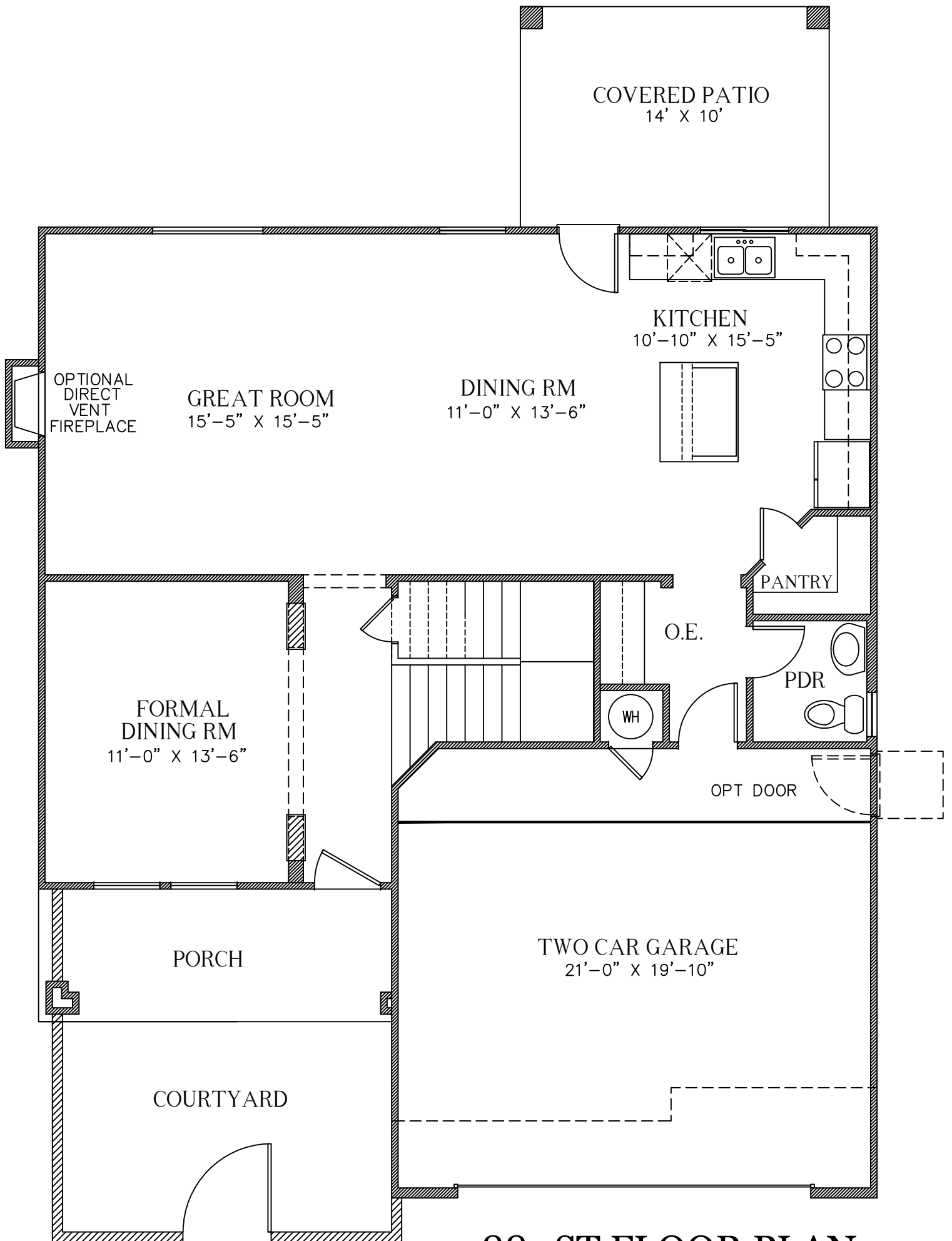
2288 1ST FLOOR PLAN
