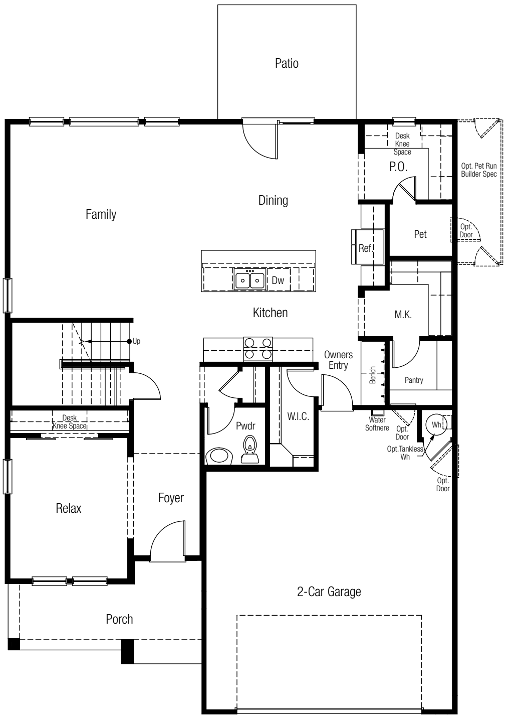
First Floor
