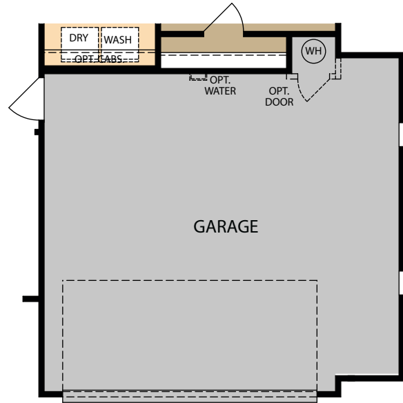
OPT. 4' SIDE GARAGE EXTENSION
