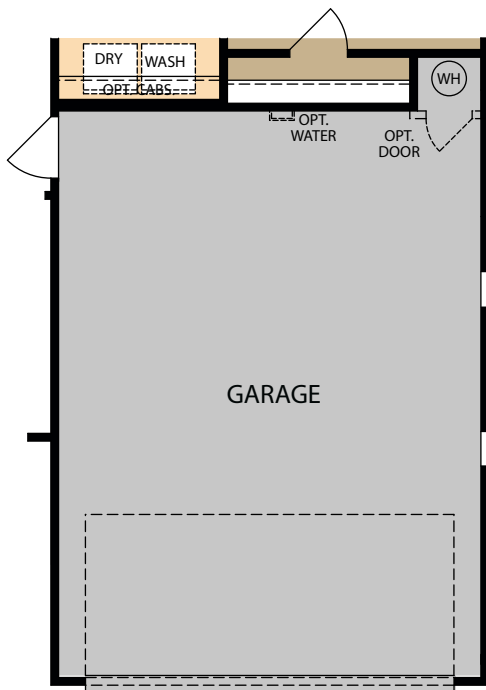
OPT. 4' FRONT GARAGE EXTENSION
