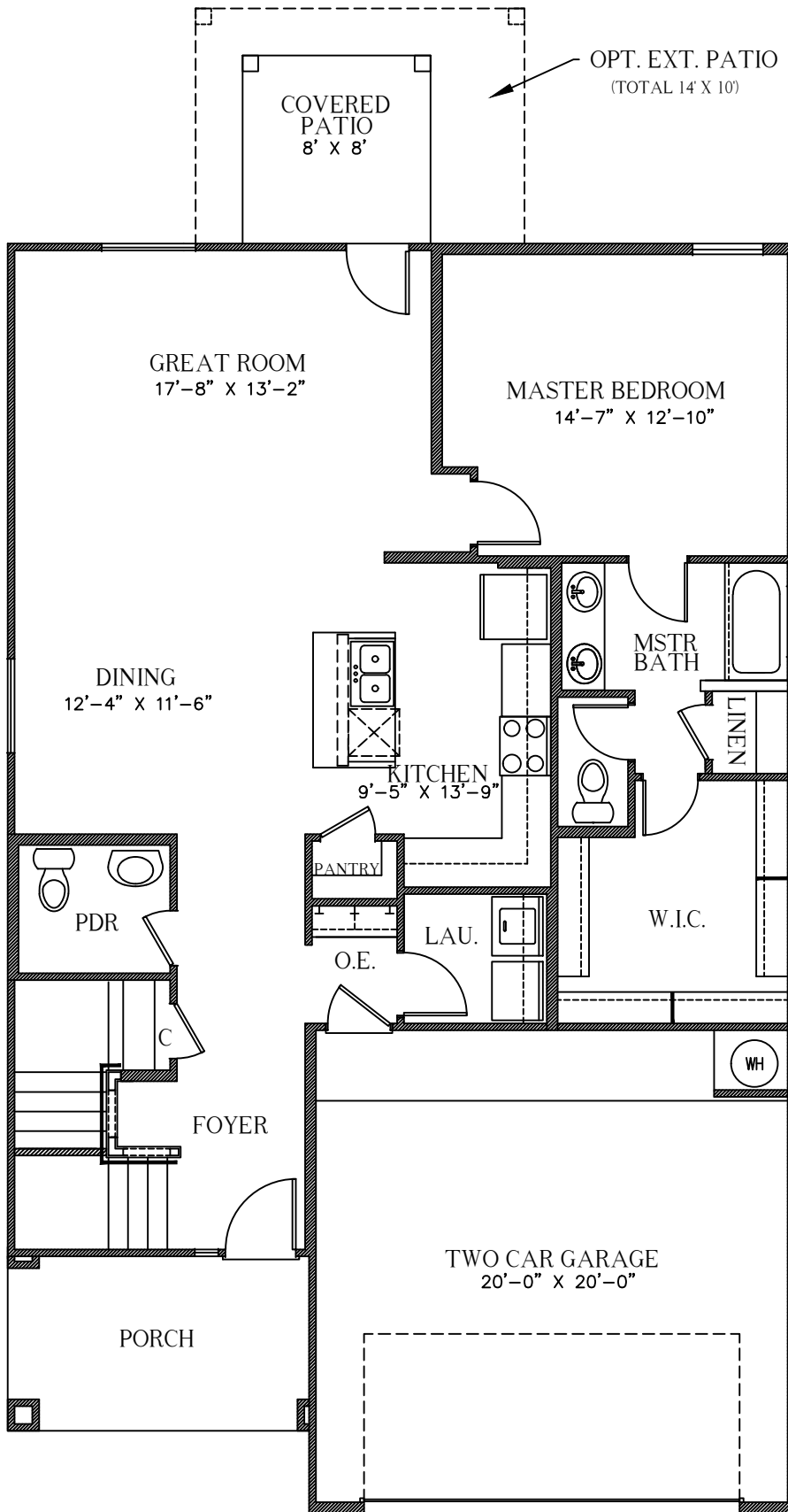
1314 1ST FLOOR PLAN
