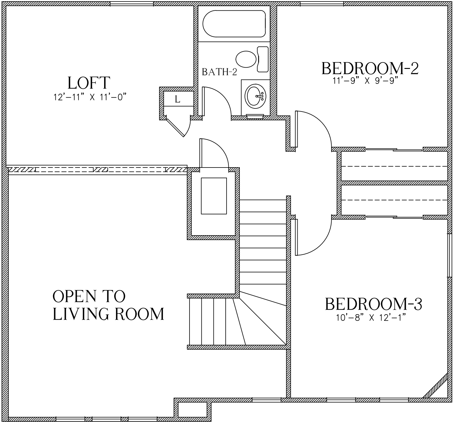
1307 2ND FLOOR PLAN
