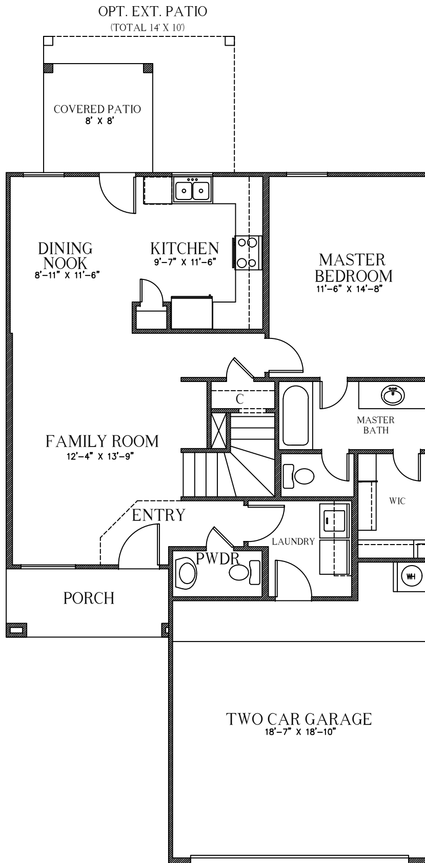
1307 1ST FLOOR PLAN
