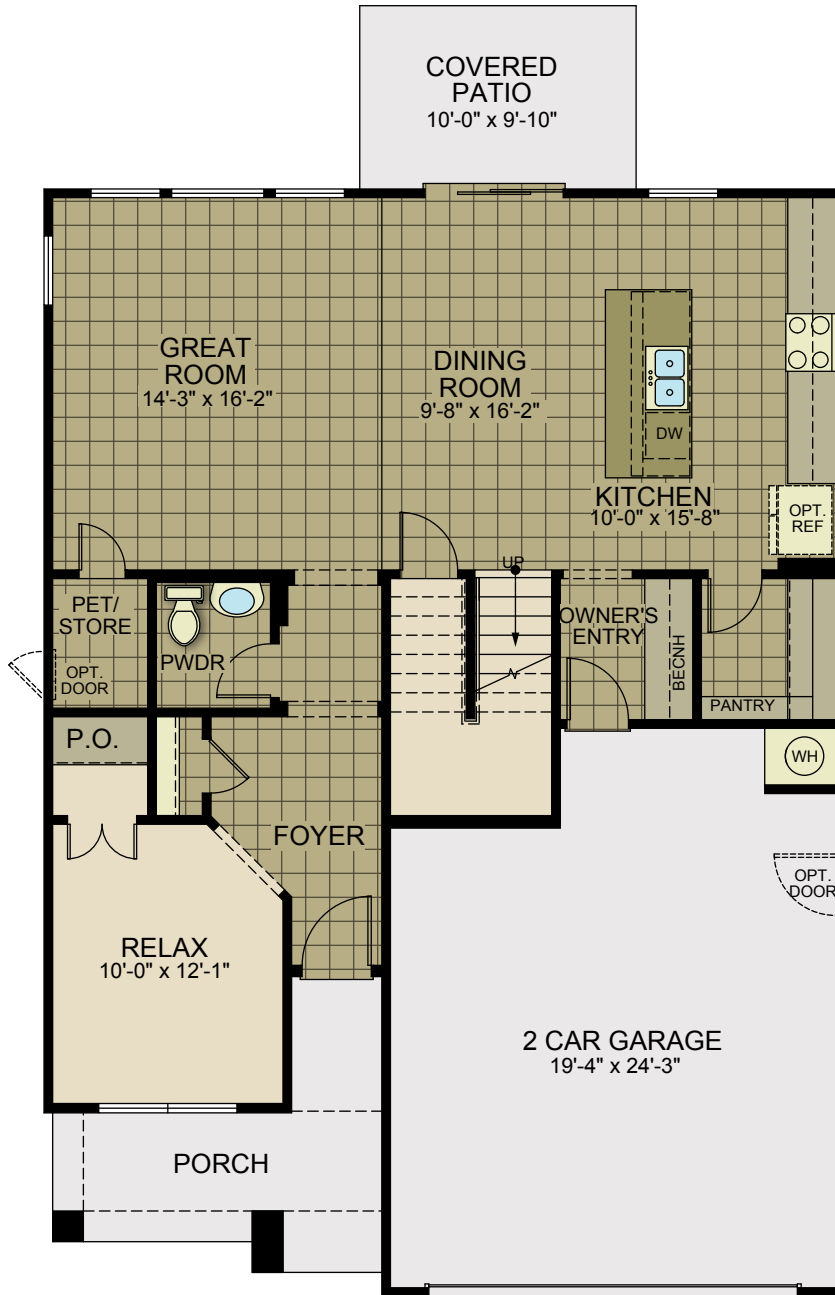
FIRST FLOOR 2,139 Sq.ft
